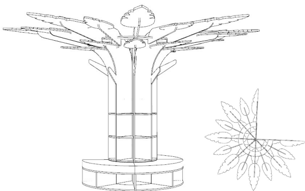
Three Quarter Tree 2400mmH x 4000mmW x 4000mmD (to leaf tip) 94.4InH x 157.4InW x 157.4InD Base dimensions: 1560mmW x 1560mmD 61.4InW x 61.4InD
