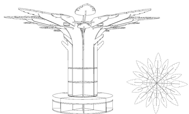
Full Circle Tree 2400mmH x 4000mmW x 4000mmD (to leaf tip) 94.4InH x 157.4InW x 157.4InD Base dimensions: 1560mmW x 1560mmD 61.4InW x 61.4InD
