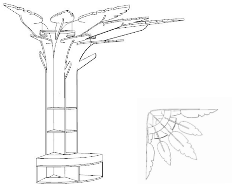
Quarter Tree 2400mmH x 2000mmW x 2000mmD (to leaf tip) 94.4InH x 78.7InW x 78.7InD Total base width: 780mmW x 780mmD 30.7InW x 30.7InD
