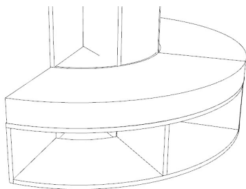
Three Quarter Tree 2400mmH x 4000mmW x 4000mmD (to leaf tip) 94.4InH x 157.4InW x 157.4InD Base dimensions: 1560mmW x 1560mmD 61.4InW x 61.4InD
