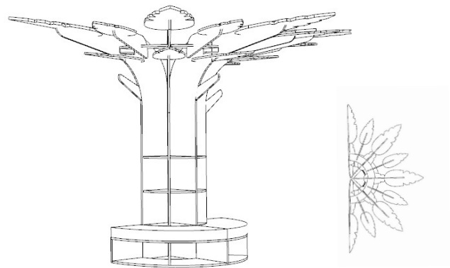
Half Tree 2400mmH x 4000mmW x 2000mmD (to leaf tip) 94.4InH x 157.4InW x 78.7InD Total base width: 1560mmW x 780mmD 61.4InW x 30.7InD
